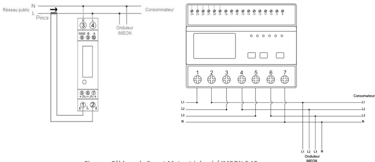
Figure - Câblage du Smart Meter triphasé / IMEON 9.12
