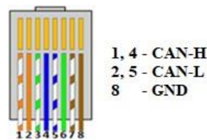
Figure - Câblage RJ45
