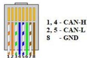
Figure 1 - RJ45 connector
