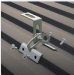
Attach the hook holder to roof slope with self-drilling screws
