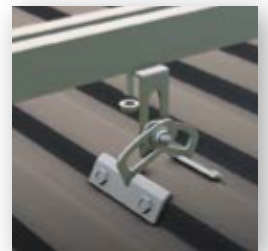
Use a flange nut serrated to connect profile with a handle
