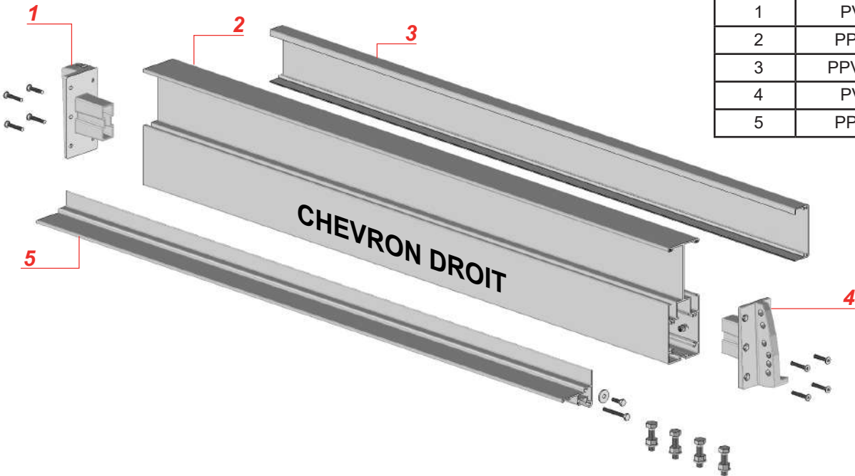
Chevron support panneau PV.
